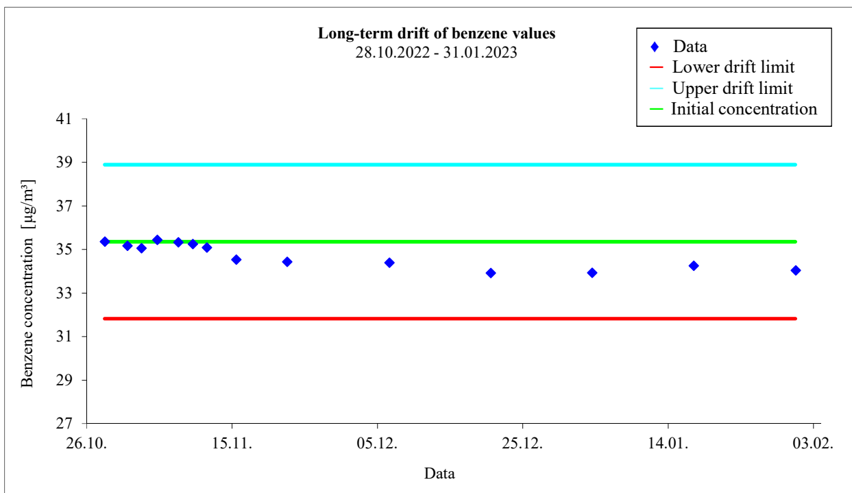
Fig. 6.3: Long term drift D_{l,s} at test value 2 (set point: 35.1 \mu\text{g}/\text{m}^3 ) - GC 80002
